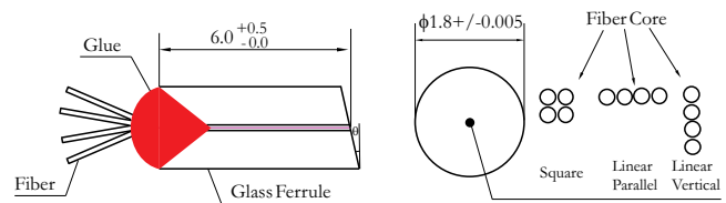
Figure 2. Four Fiber Pigtail
